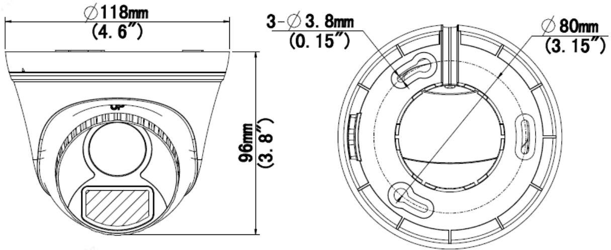
UAC-T115-F28(40)-W
